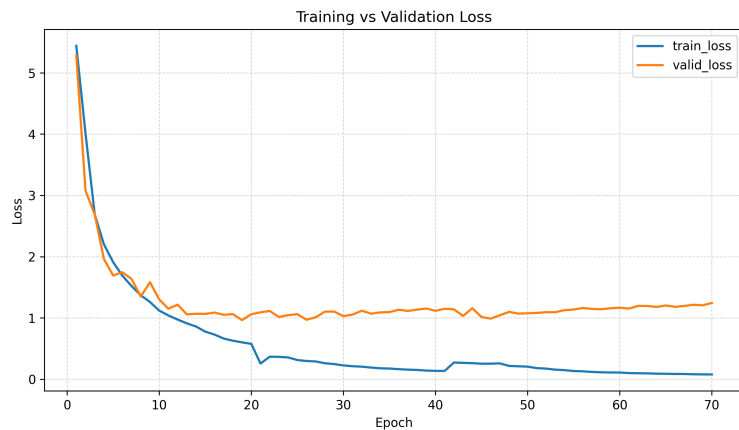
Figure 1.5 Training vs validation loss
